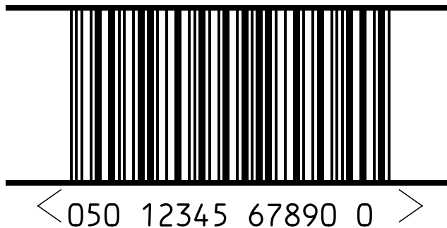
ITF-14 bar code with X-dimension of 0.495 mm
