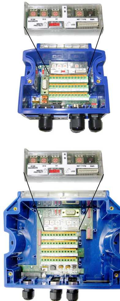
Figure 2 – BM100 Mounting
