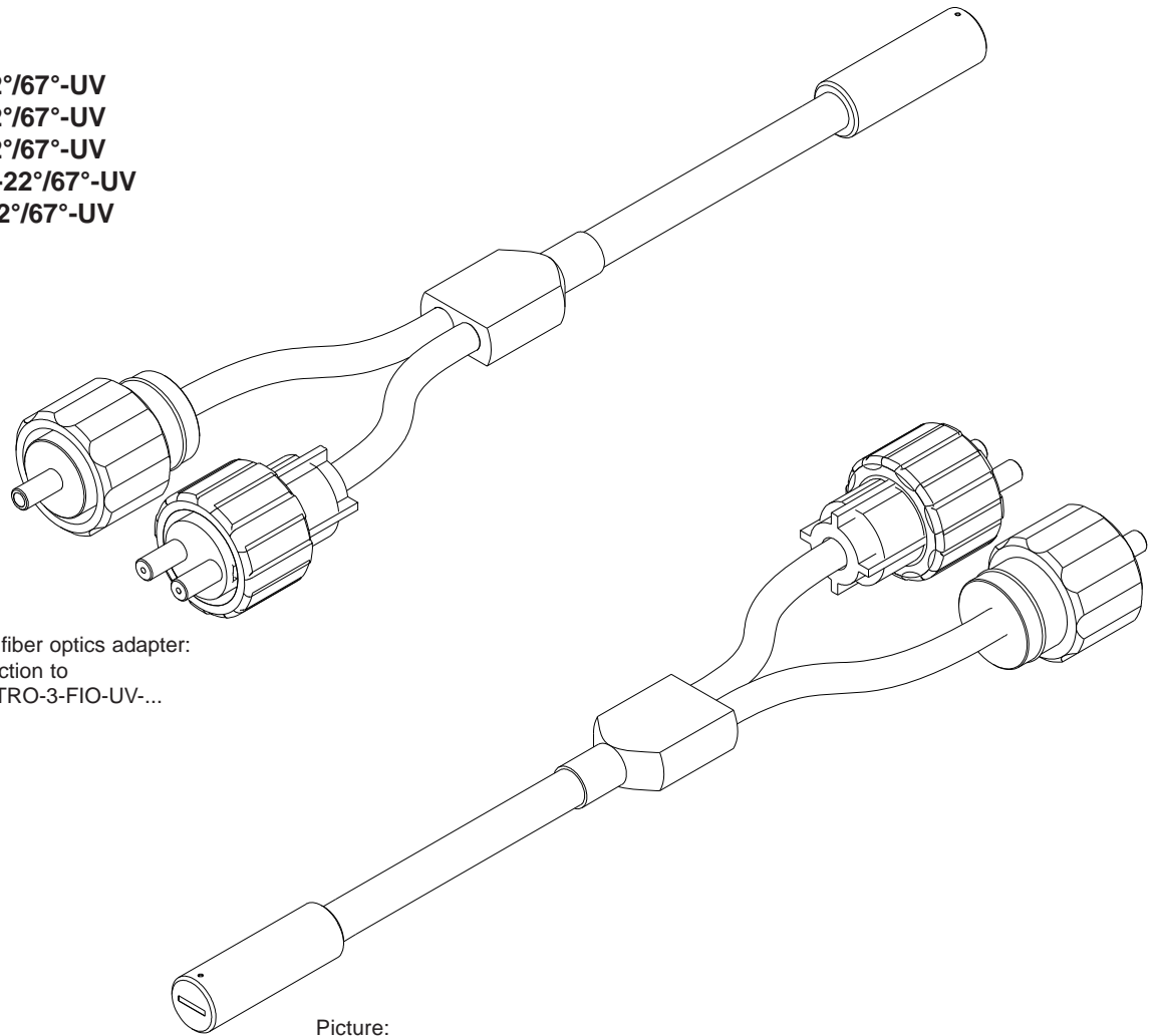
Picture: R-S-R2.1-(6x1)-1200-Y-22°/67°-UV
