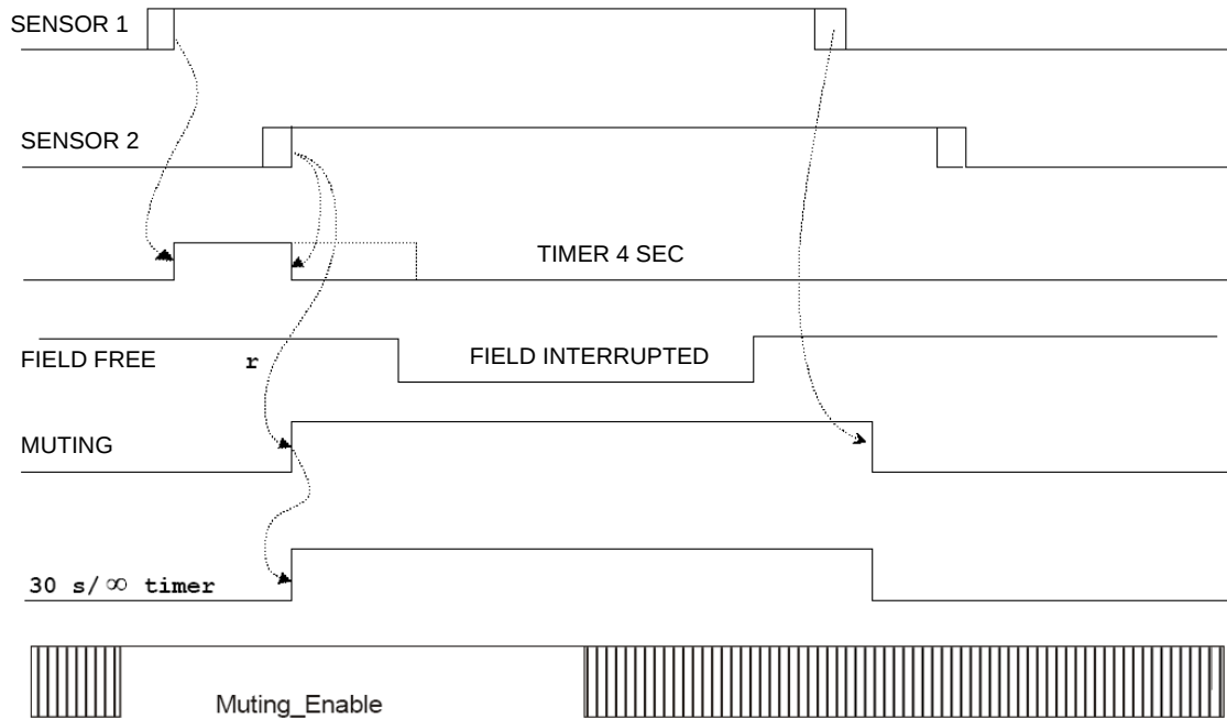
Figure 12 Muting cycle
